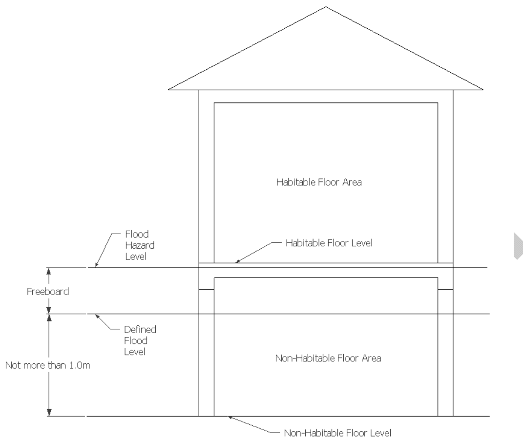
Figure C2.6 Elevation showing DFL
